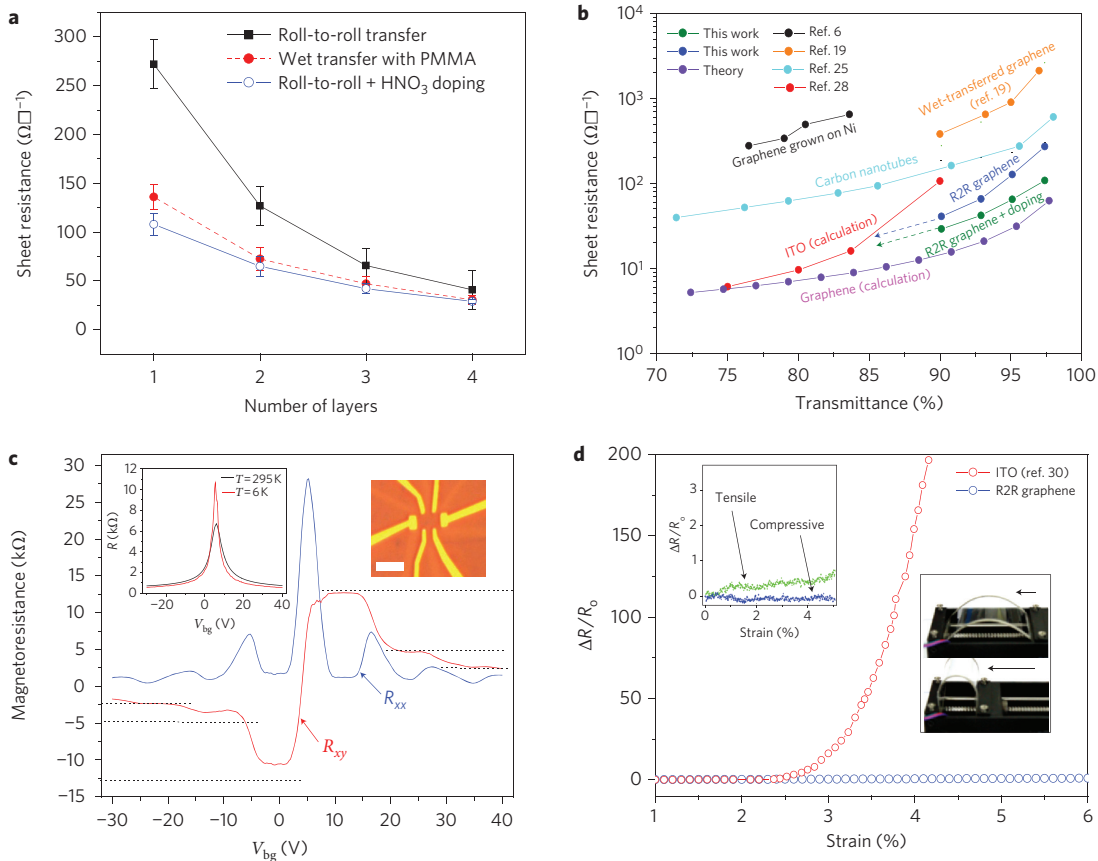
Figure 4 | Electrical characterizations of layer-by-layer transferred and HNO 3 -doped graphene films. a , Sheet resistances of transferred graphene films using a roll-to-roll (R2R) dry-transfer method combined with thermal release tapes and a PMMA-assisted wet-transfer method. b , Comparison of sheet resistance from this research and transmittance plots taken from other references. The dashed arrows indicate the expected sheet resistances at lower transmittance. The scheme is borrowed from ref. 19. c , Electrical properties of a monolayer graphene Hall bar device in vacuum. Four-probe resistivity (left bottom inset) is measured as a function of gate voltage in the monolayer graphene Hall bar shown in the right inset at room temperature (black curve) and T = 6 K (red curve). The QHE effect at T = 6 K and B = 9 T is measured in the same device. The longitudinal resistivity \rho_{xx} and Hall conductivity \sigma_{xy} are plotted as a function of gate voltage. The sequence of the first three half-integer plateaus corresponding to \nu = 2, 6 and 10 , typical for single-layer graphene, are clearly seen. The Hall effect mobility of this device is \mu_{\text{Hall}} = 7,350 \text{ cm}^{-2} \text{ V}^{-1} \text{ s}^{-1} at 6 K ( \sim 5,100 \text{ cm}^{-2} \text{ V}^{-1} \text{ s}^{-1} at 295 K). Scale bar (inset), 3 \mu\text{m} . d , Electromechanical properties of graphene-based touch-screen devices compared with ITO/PET electrodes under tensile strain. The inset shows the resistance change with compressive and tensile strain applied to the upper and lower graphene/PET panels, respectively.
